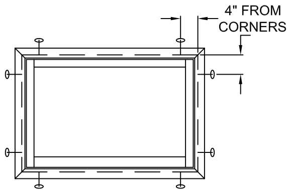
TYPICAL ELEVATION WITH FASTENER SPACING
